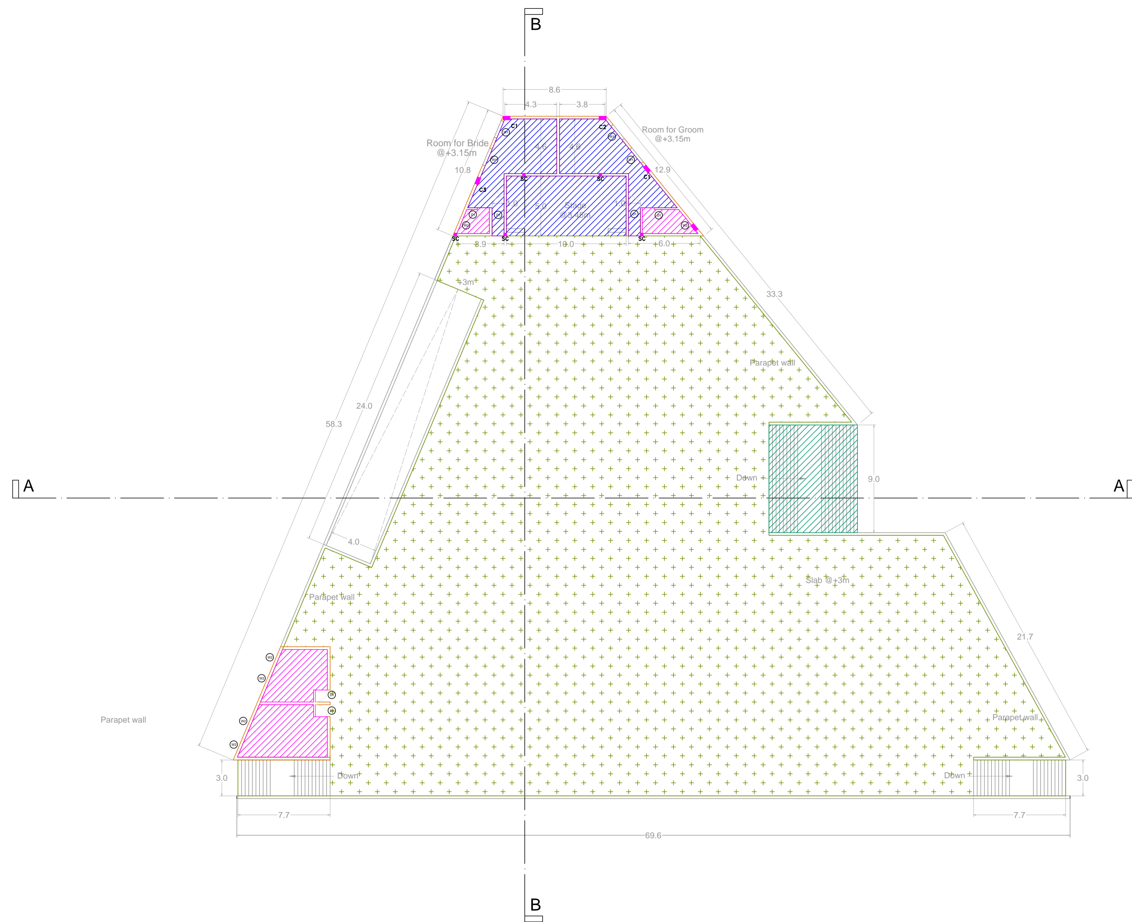
1ST FLOOR PLAN @ +3.0M
