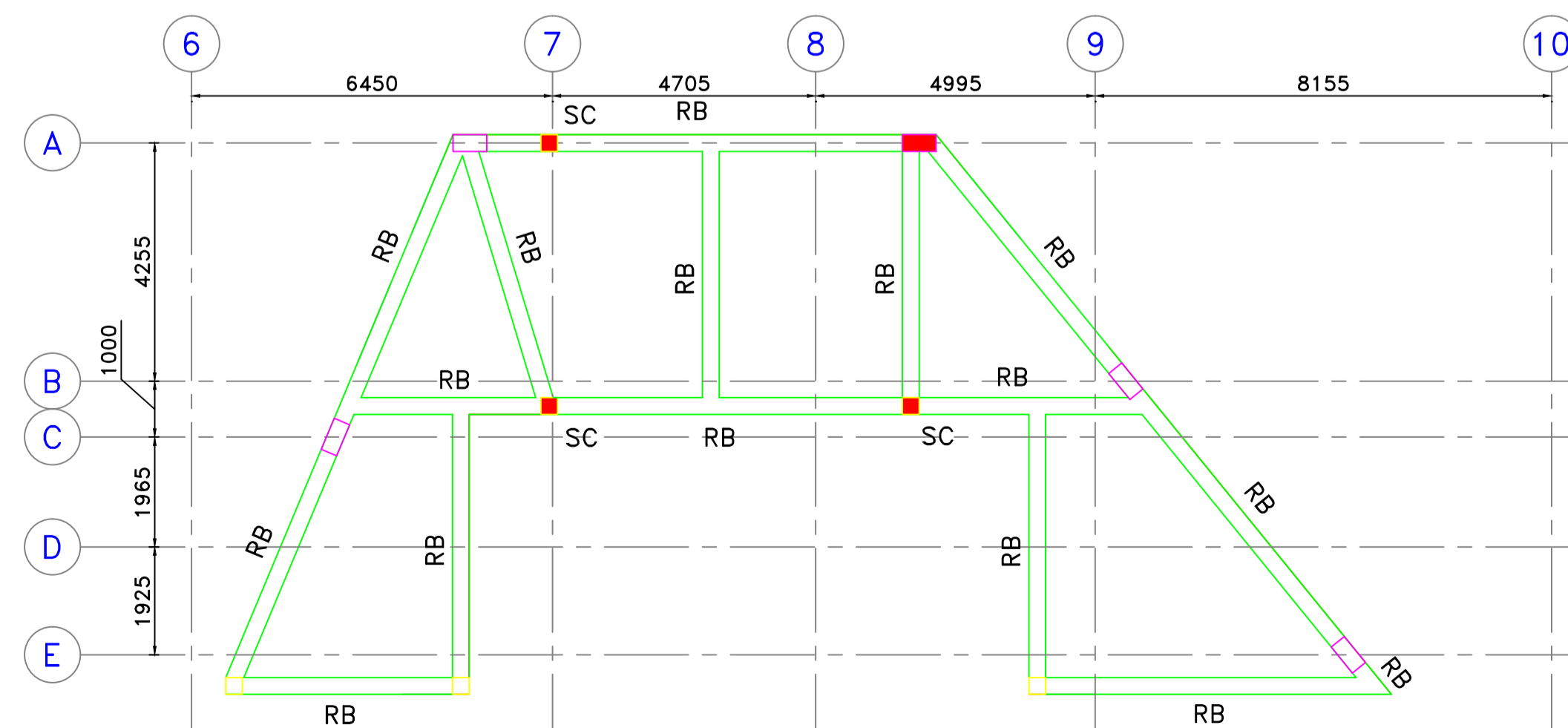
LAYOUT OF ROOF LEVEL BEAMS & SLABS AT EL(+) 5.950M ALL BEAMS ARE 300MM WIDE & 600MM DEEP THICKNESS OF SLAB IS 125MM
