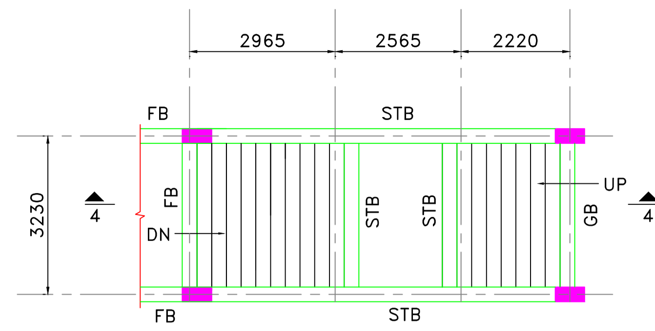
LAYOUT OF STAIRCASE-1&2 ALL BEAMS ARE 300MM WIDE & 600MM DEEP THICKNESS OF FLIGHT SLAB IS 150MM
