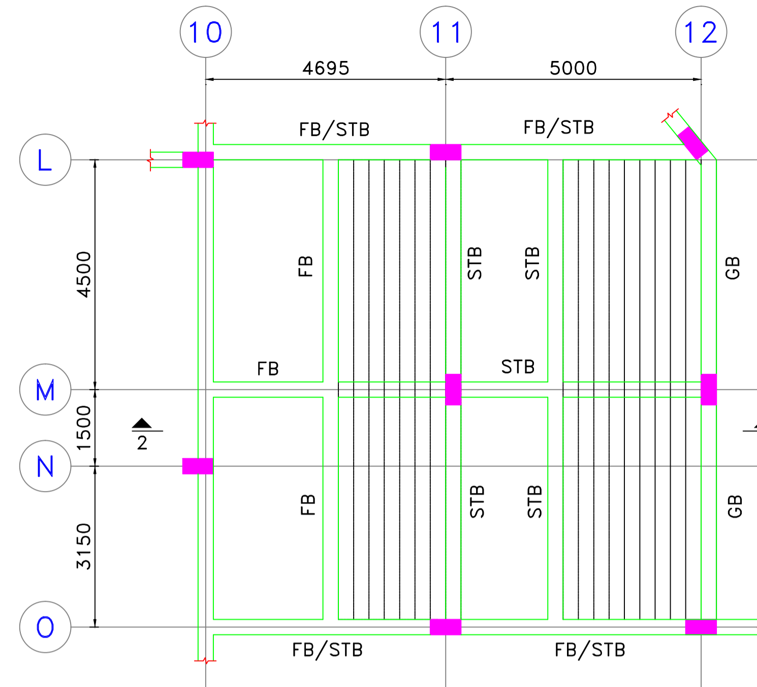
LAYOUT OF STAIRCASE-3 ALL BEAMS ARE 300MM WIDE & 600MM DEEP THICKNESS OF FLIGHT SLAB IS 150MM
