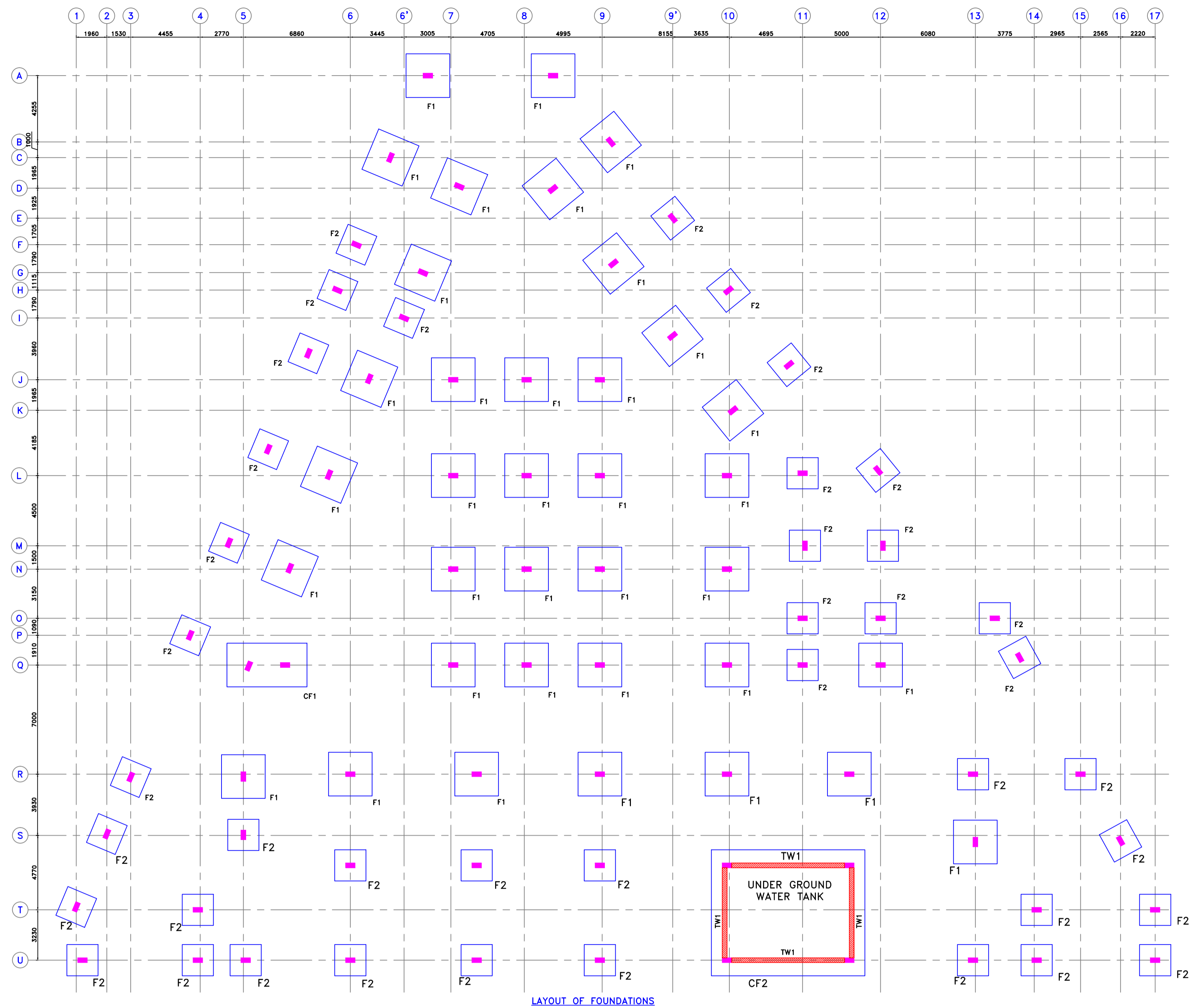
LAYOUT OF FOUNDATIONS
