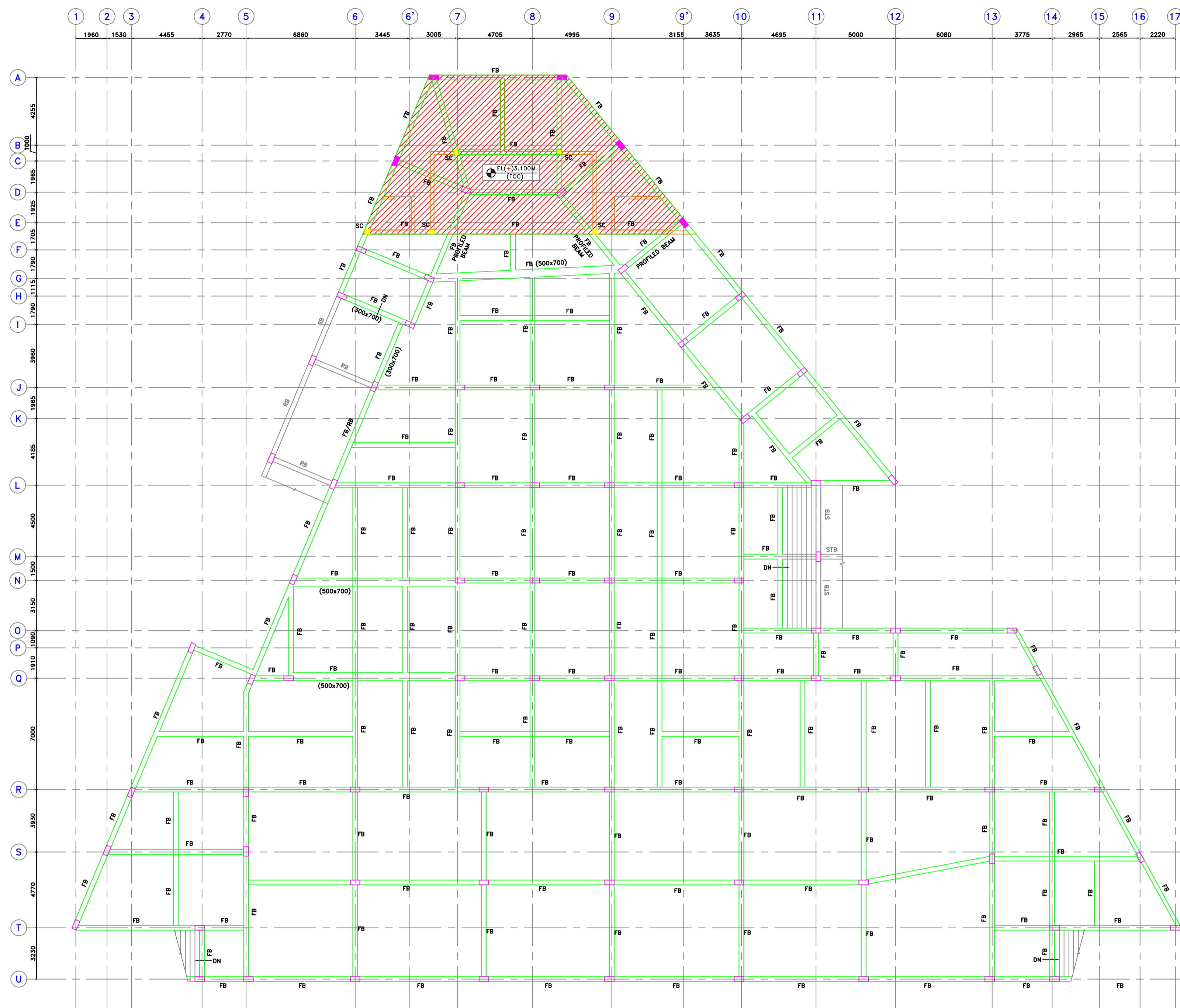
LAYOUT OF FIRST FLOOR BEAMS & SLABS AT EL(+) 2.950M ALL BEAMS ARE 300MM WIDE & 600MM DEEP, UNO THICKNESS OF SLAB IS 150MM
