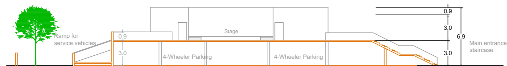
SECTION AA
