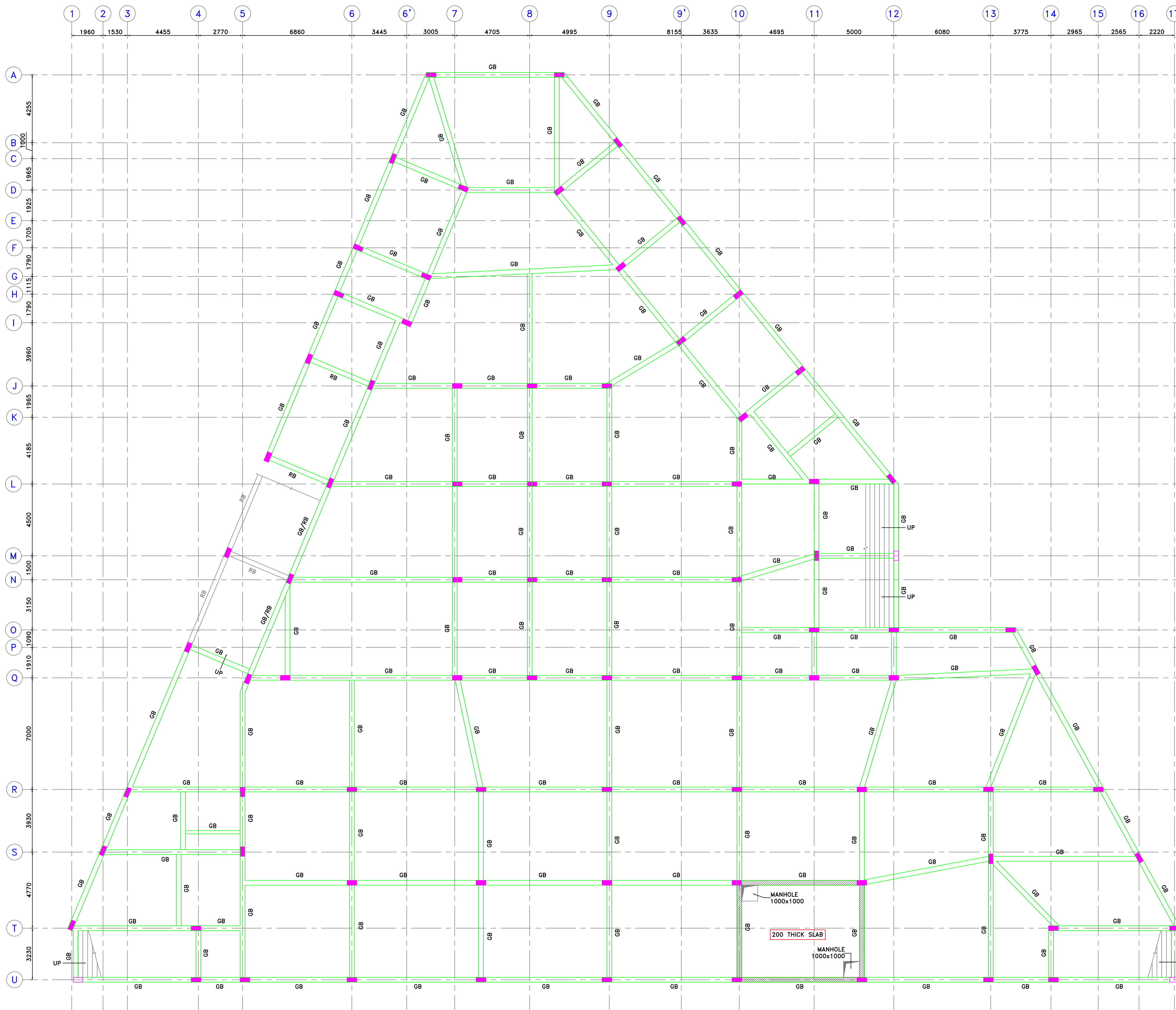
LAYOUT OF GROUND FLOOR LEVEL BEAMS AT EL(-)0.50M (TOC),UNO ALL BEAMS ARE 300MM WIDE & 600MM DEEP
